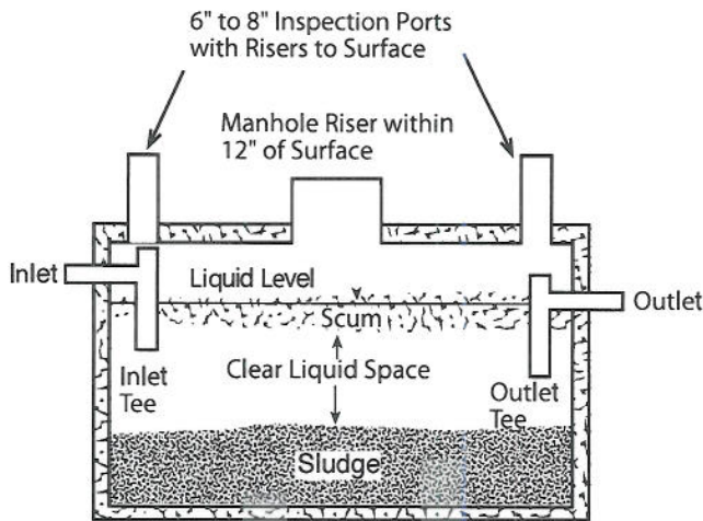
Figure 2. A septic tank designed for easy maintenance.
