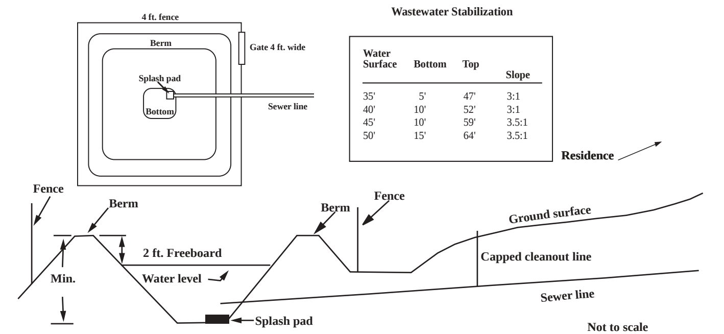
Figure 2. Wastewater lagoon plan, dimensions and cross-section
